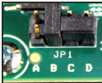
Image 1 : Avid Delay Matching Jumper installed on B
